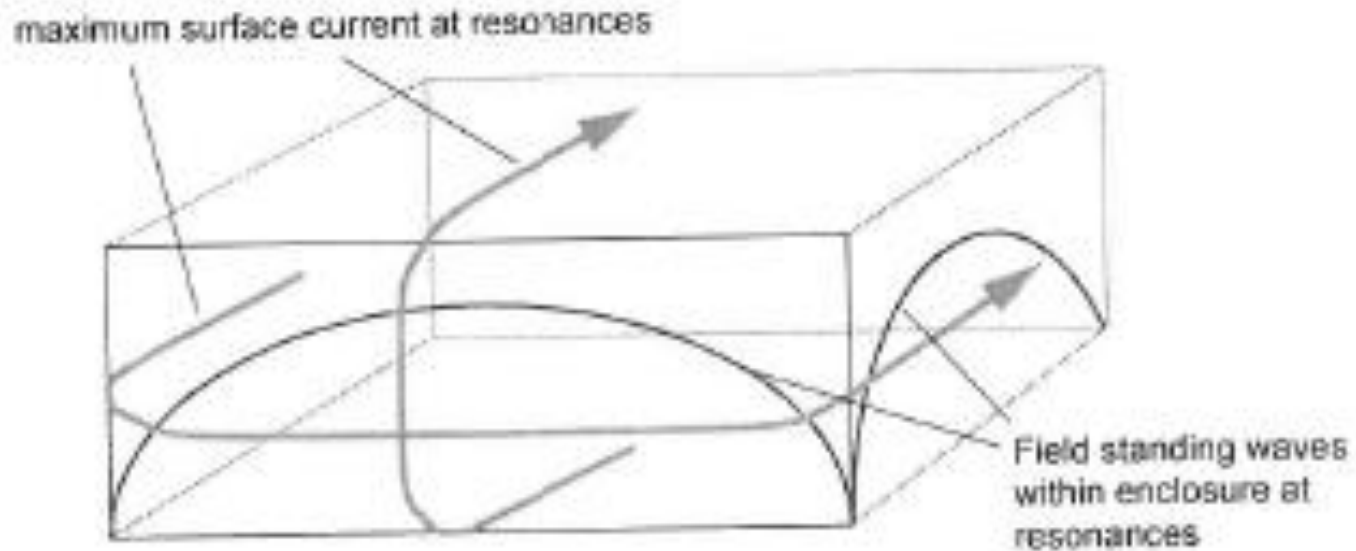
Figure 14.4 Resonances degrade shielding effectiveness
