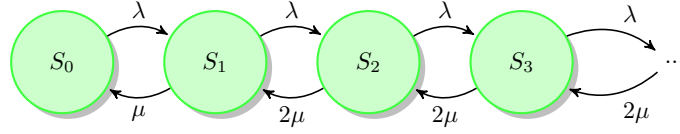
Figure 13: System diagram for the second model of exercise 7.2
