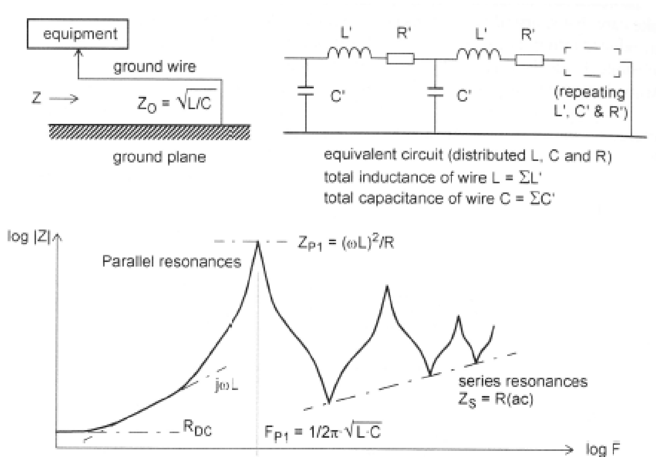
Figure 11.7 The impedance of long ground wires
