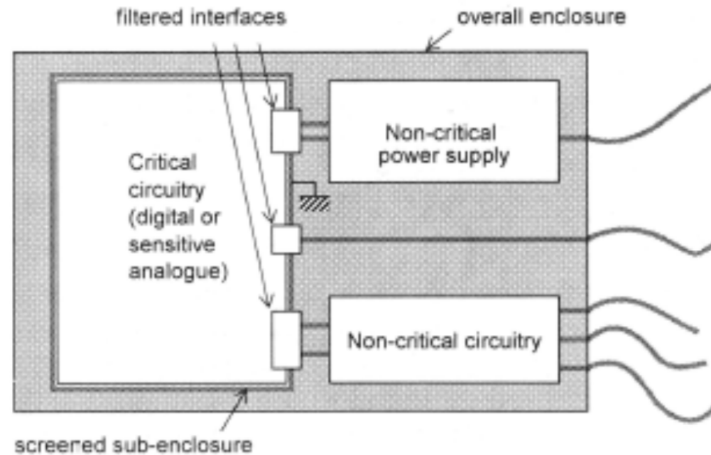
Figure 11.3 System partitioning
