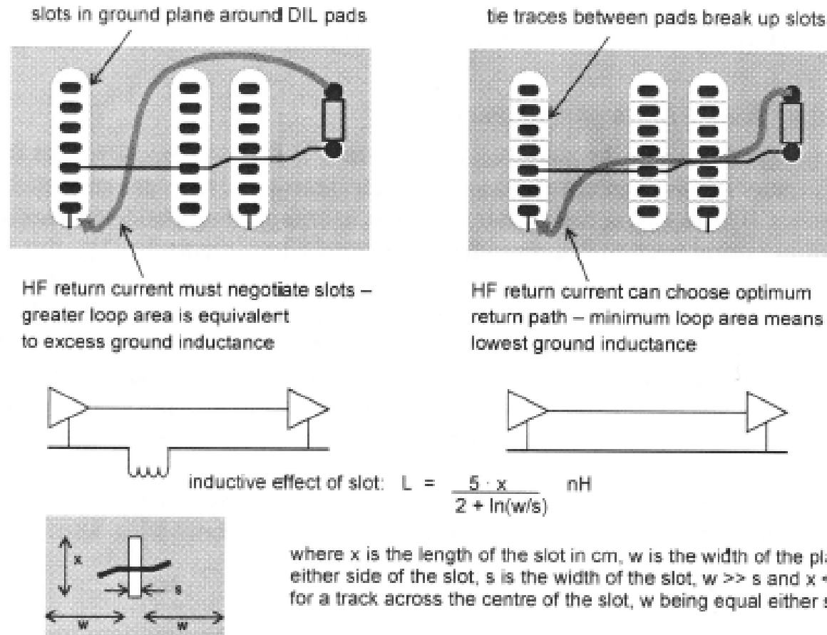
Figure 11.16 Dealing with slots at DIL pinouts
