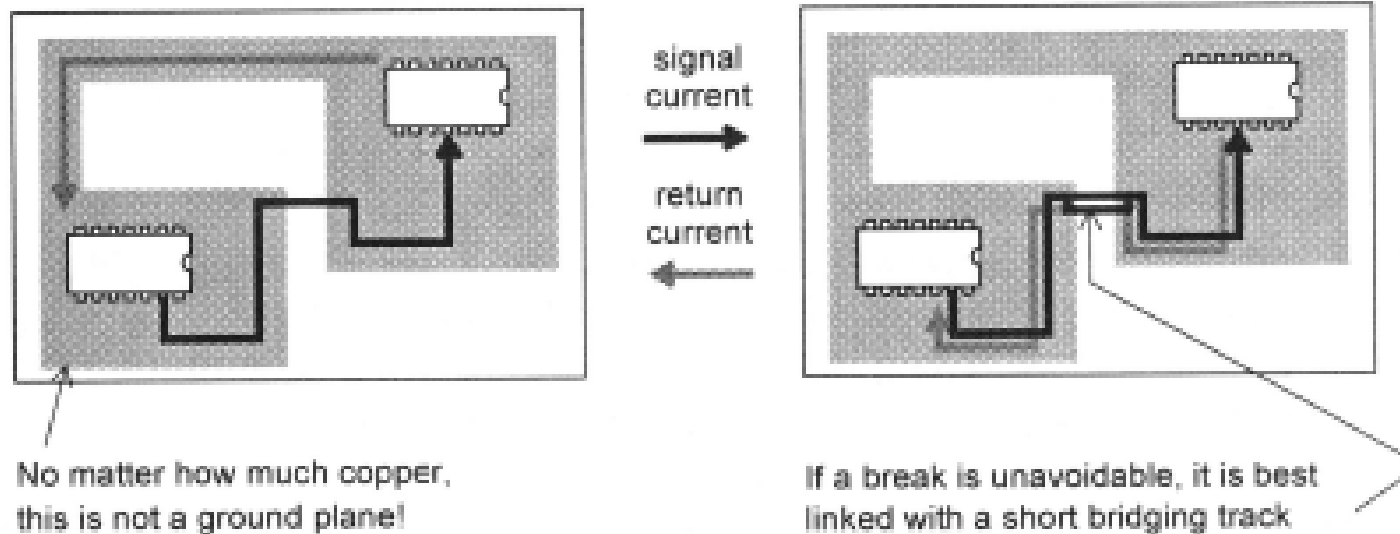
Figure 11.15 A broken ground plane
