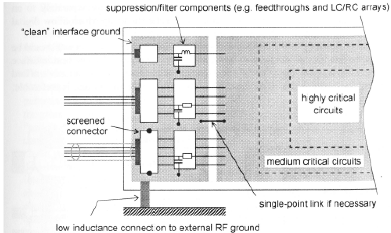
Figure 11.23 The interface ground on a PCB
