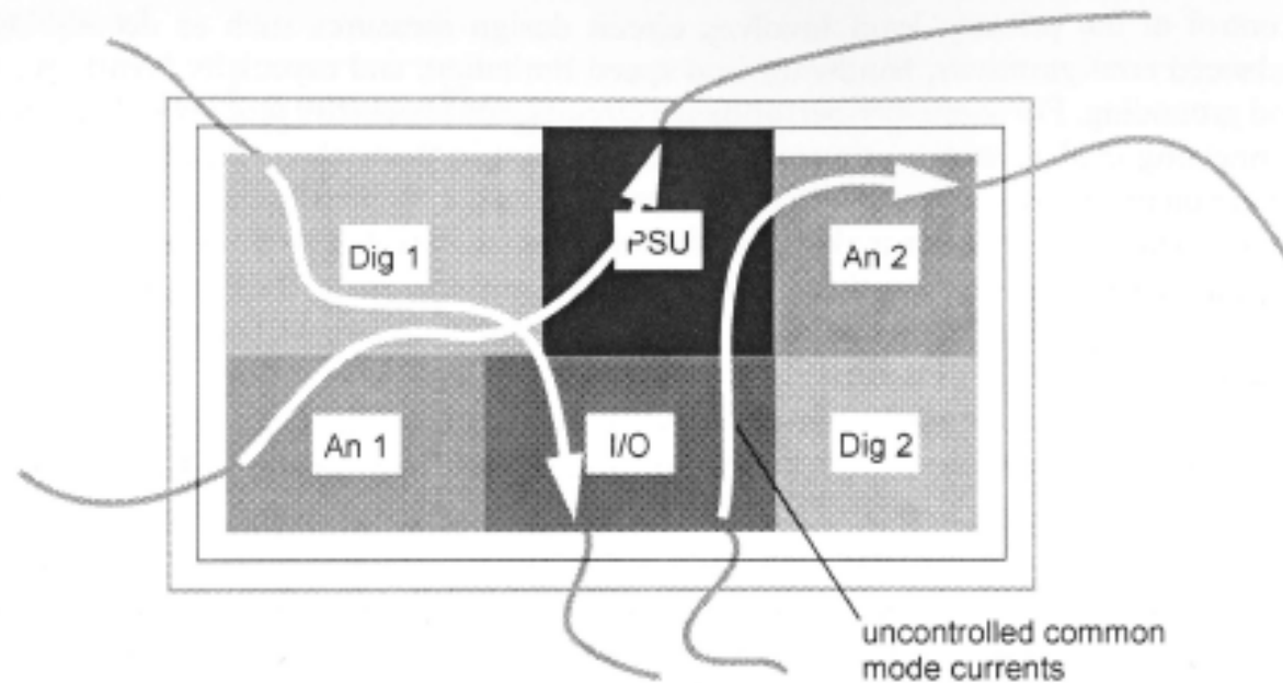
Figure 11.2 The haphazard system
