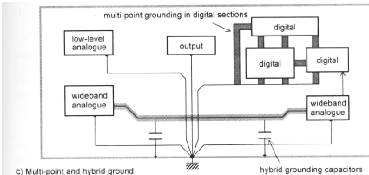
Figure 11.6 Grounding systems
