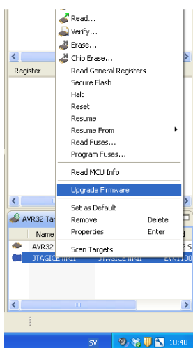
Upgrade Firmware
