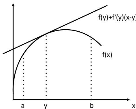
Figure 8.1: The tangent line f(y) + f'(y)(x - y) at y \in [a, b] .
