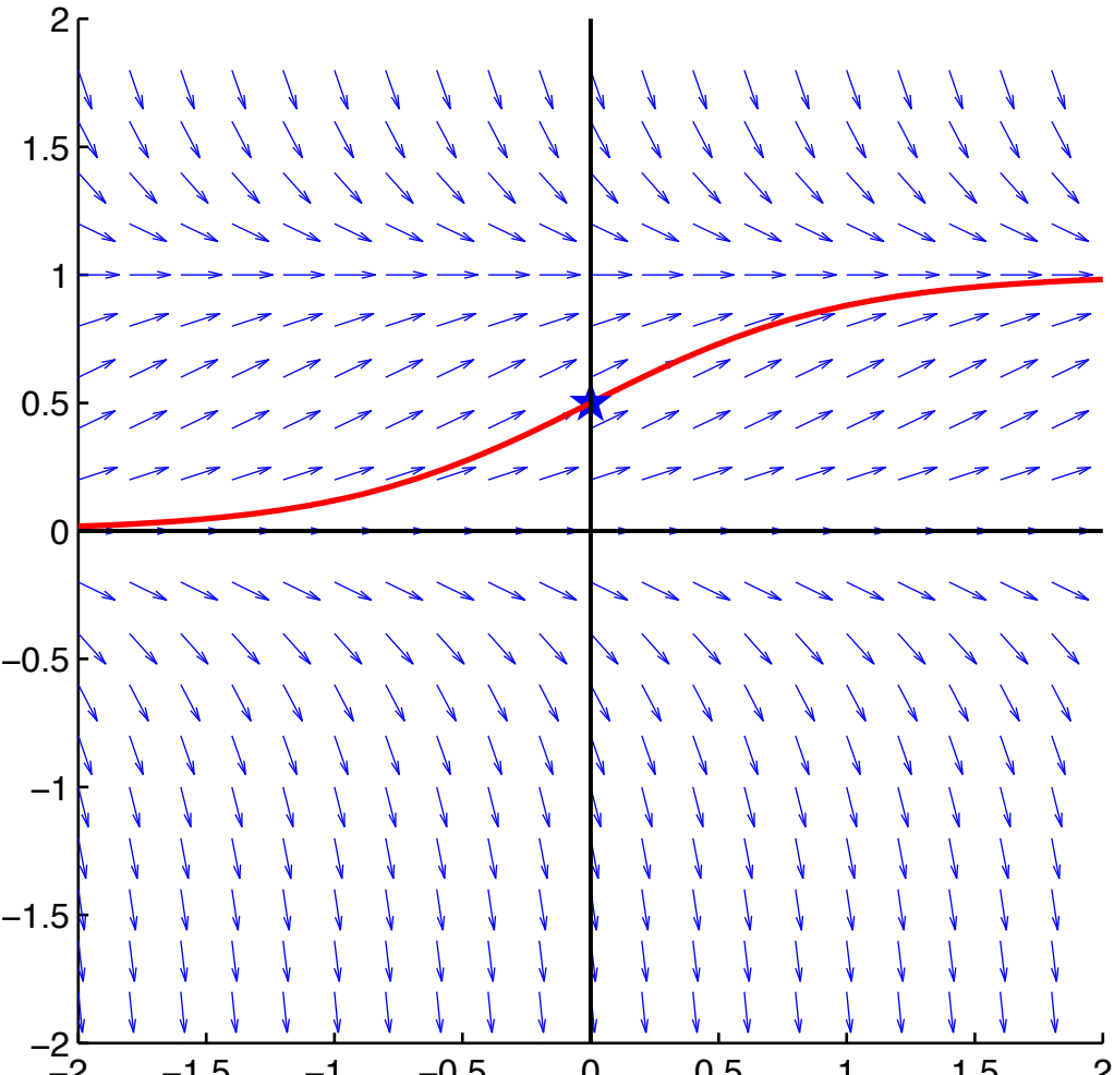
fig160509(1): y'=2*y*(1-y)
