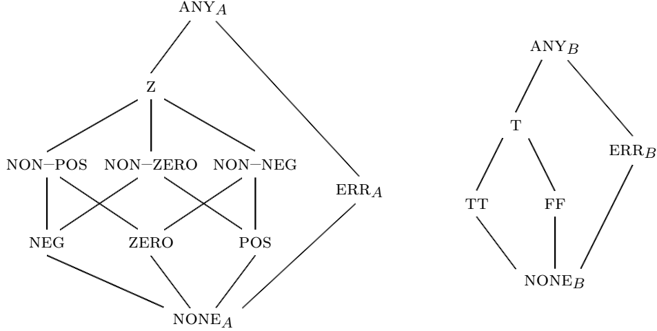
Figure 1: The lattices for SignExc and TTEnc .
