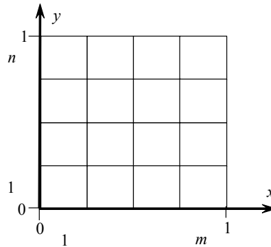
Figure 1: Finite volume grid
