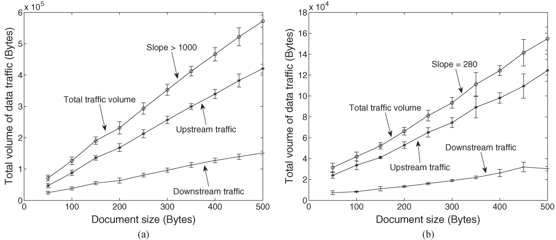
Fig. 4. Volume of traffic generated vs the size of the document for (a) Google Drive and (b) Microsoft Skydrive word processing applications.
