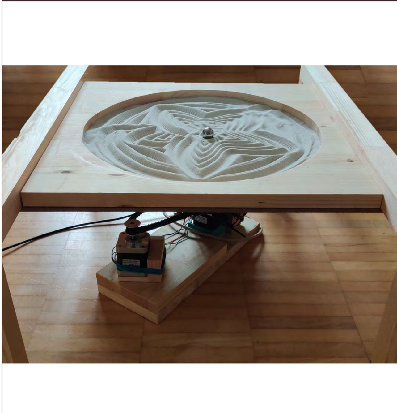
Final build for the sand table. The patterns can be set from a computer.
