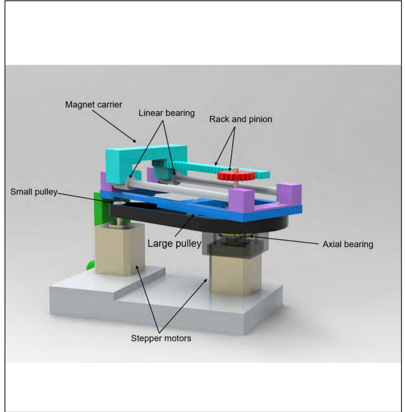
The final prototype in Solid edge.
