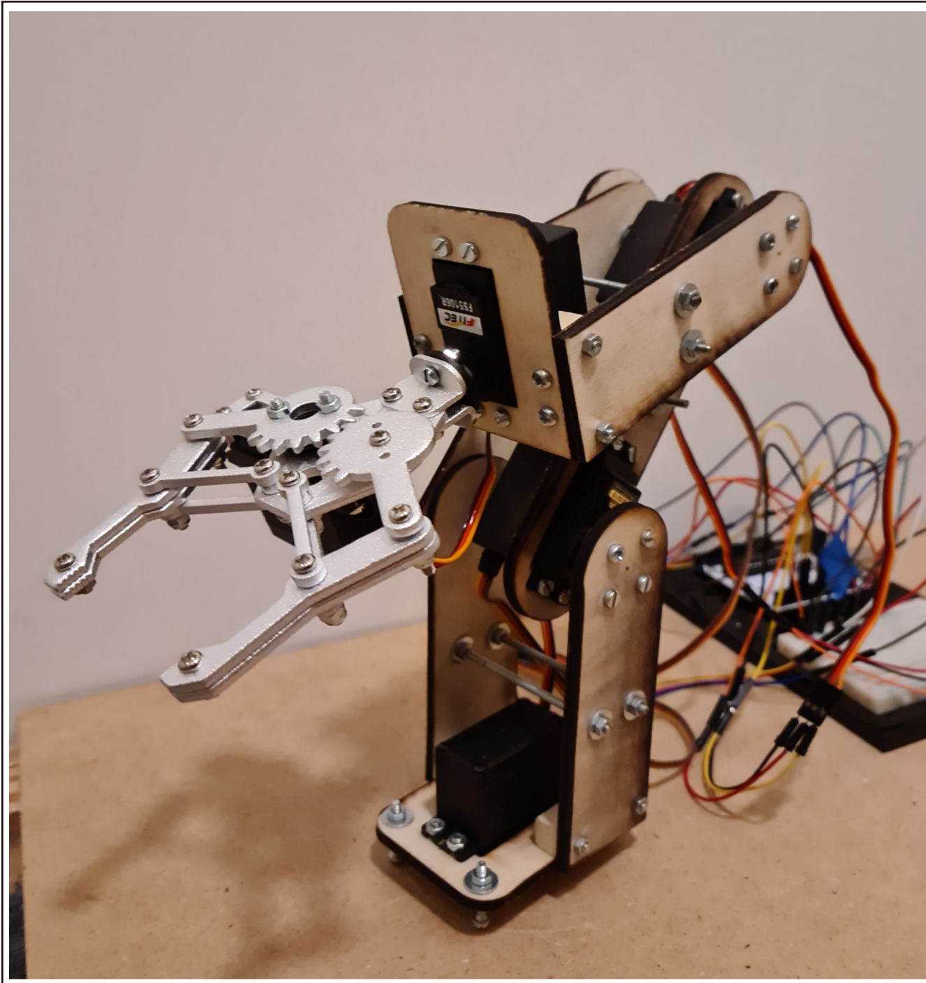
Final model of the robotic arm
