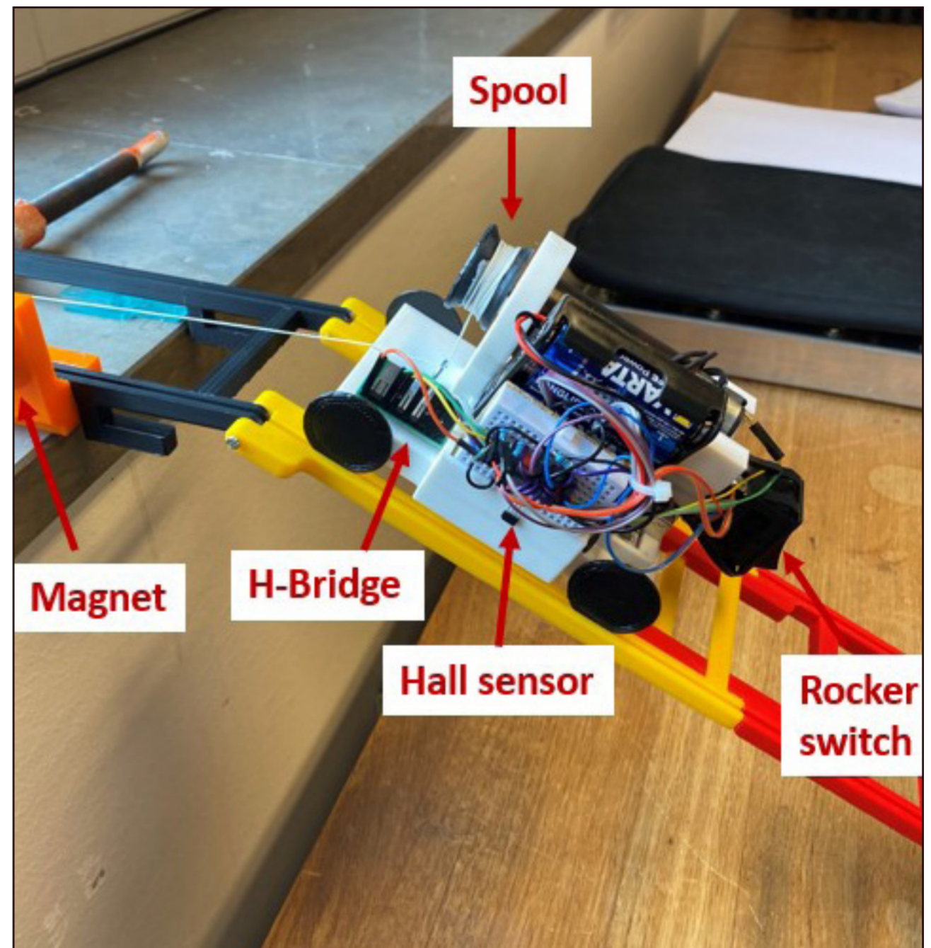
The prototype utilizes an H-Bridge and a Hall sensor to run, stop and reverse.
